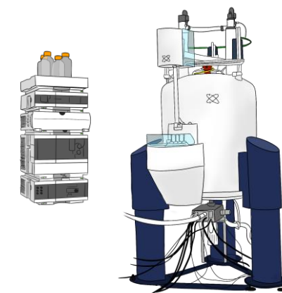
Structural Determination (NMR, GC/LC-MS, X-Ray)
