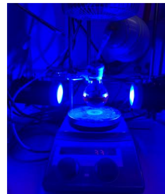
Photochemical Set-Up and Photocatalysts
