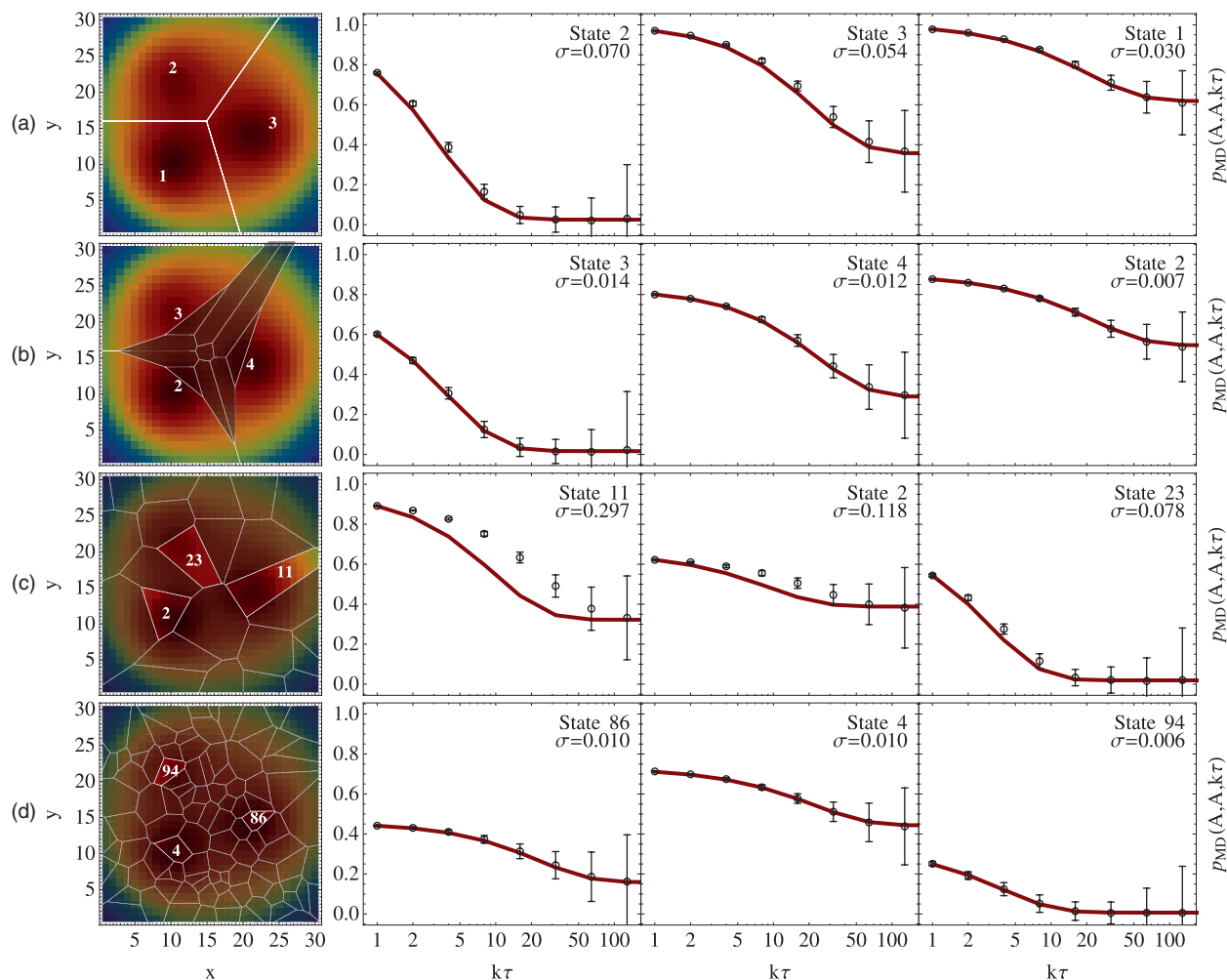
FIG. 12. Chapman–Kolmogorov test for the three-well diffusion model (see also Fig. 6). For each of four discretizations (first column, a, b, c, d), the Chapman–Kolmogorov test is shown for the three states with the greatest error (labeled with white figures in the first column). Relaxation curves from a 250 000 step trajectory, p_{MD}(A, A; k\tau) (black) along with the uncertainties \epsilon_{MD}(A, A; k\tau) are compared to the model prediction, p_{MSM}(A, A; k\tau) (red). The total error \sigma given in the top right corners is measured as the 2-norm of the vector containing the differences p_{MD}(A, A; k\tau) - p_{MSM}(A, A; k\tau) for time points in the range k\tau \in [1, 128] .
