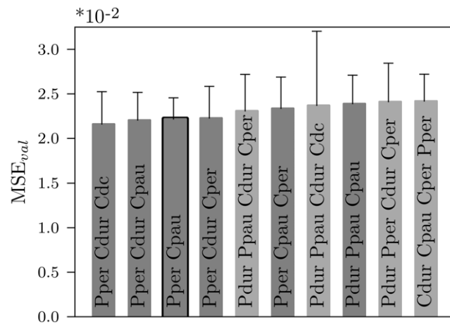
Figure 4. Ten best performing models. Model of size four (light gray), three (dark gray), and two (black edging) are ranked top ten. The overall best performing model uses the pulse period, chirp duration, and chirp duty cycle. The best 2-feature model (pulse period and chirp pause) did not perform significantly different ( p -value=0.028 for a two-sided Wilcoxon rank-sums test; significance level of 0.01). The best 4-feature model (pulse duration, pulse pause, chirp duration, and chirp period) performed significantly worse than the best 3-feature model ( p -value<0.01 for a two-sided Wilcoxon rank-sums test). Abbreviations: Pdur - pulse duration, Ppau - pulse pause, Pper - pulse period, Pdc - pulse duty cycle, Cdur - chirp duration, Cpau - chirp pause, Cper - chirp period, Cdc - chirp duty cycle. The models were validated 100 times and errorbars indicate standard deviation. doi:10.1371/journal.pone.0055349.g004
