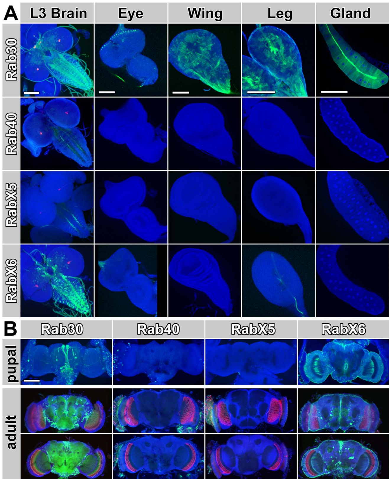
Figure 2. Cellular Expression Analysis of rab30-Gal4 , rab40-Gal4 , rabX5-gal4 and rabX6-Gal4 . All rab-Gal4 lines were crossed to UAS-CD8-GFP . (A) Larval tissues showing GFP expression in green, 3×P3-RFP (positive marker of the Gal4 knock-in cassette) and nuclear Toto3 in blue. (B) Pupal (P+30% \pm 5%) and 1-day adult brains (top panel: anterior; bottom panel: posterior). All scale bars represent 100 \mu m. doi:10.1371/journal.pone.0040912.g002
