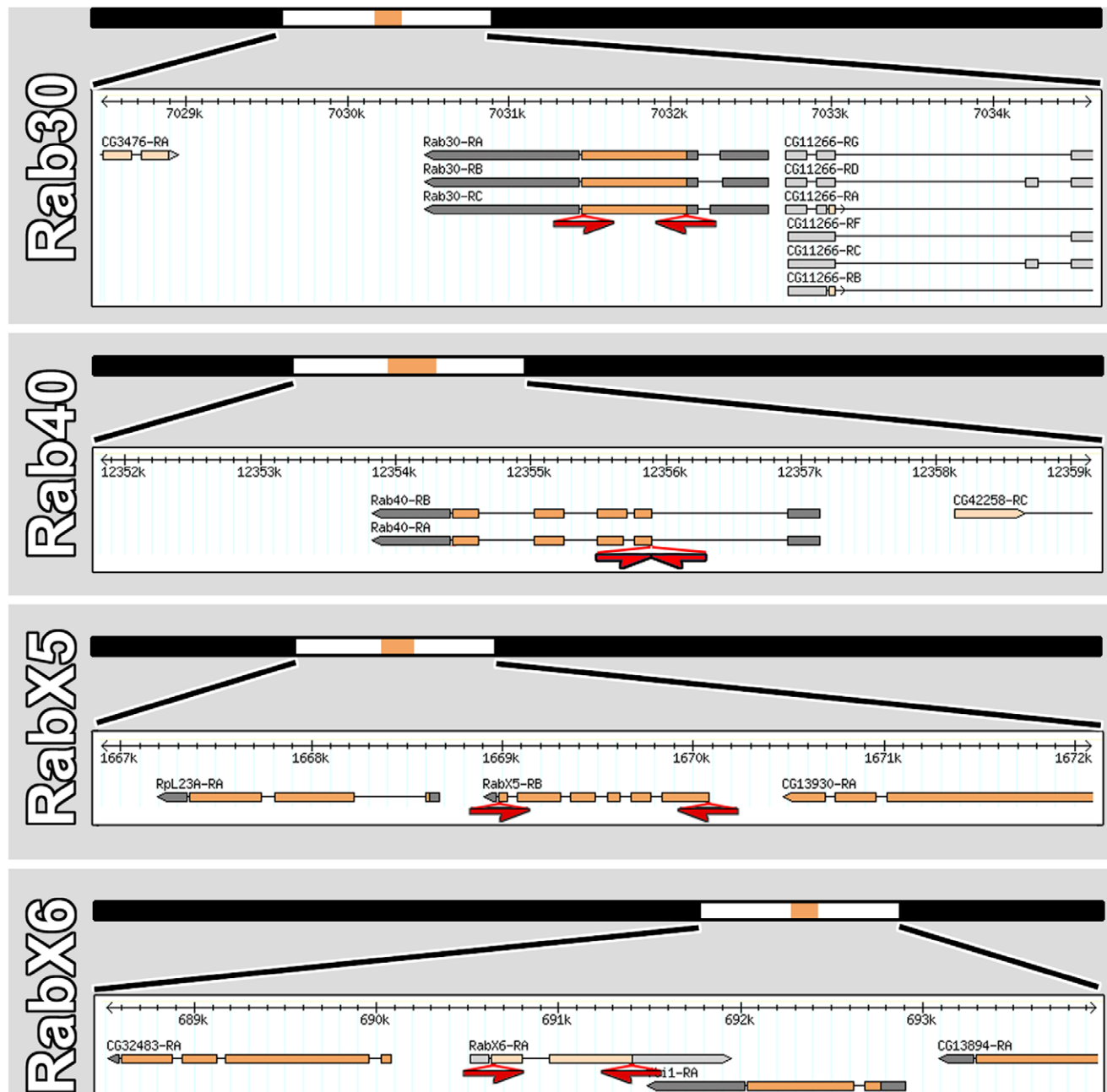
Figure 1. Targeting vector design for rab30-Gal4 , rab40-Gal4 , rabX5-Gal4 and rabX6-Gal4 . 20–22 kb genomic regions (black bars) were recombined from bacterial artificial chromosomes (BACs) into attB-P[acman]-KO [17,22]. Regions of a few kb are shown at higher resolution to reveal the structures of rab loci within these genomic regions. Sequences between red arrows were replaced with a Gal4 knock-in cassette [17]. For expression analyses, transgenic flies with the targeting vectors inserted in the same landing site were used. doi:10.1371/journal.pone.0040912.g001
