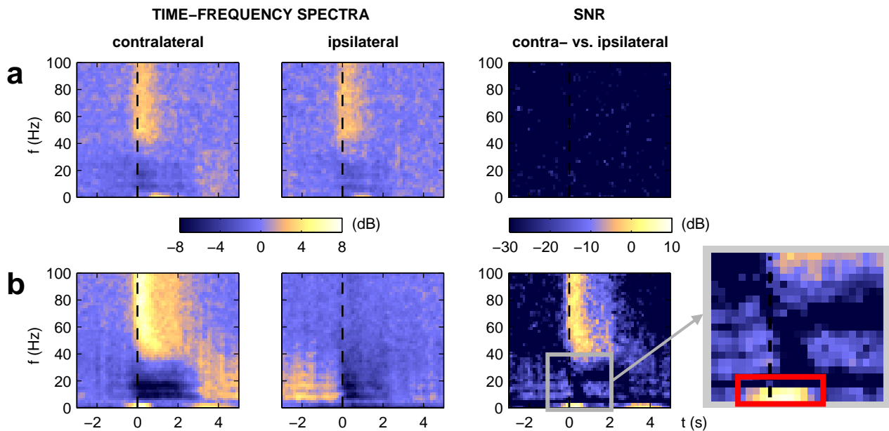
Figure 2: Time-frequency analysis of movement related epicortical potentials for two electrodes placed on (a) the premotor cortex and (b) the arm area of primary motor cortex (M1). Baseline normalized amplitude spectra (left two columns) for both electrodes showed task related spectral power changes in alpha, beta, gamma, and the low-frequency components. Significant differences between movements of the ipsi- and contralateral finger in the signal-to-noise ratio (SNR, right column) plots were observed in electrode (b), but not in (a). The box in the lower part of the magnified SNR plot marks the low-frequency SNR peak corresponding to the signal component we used for movement inference.
